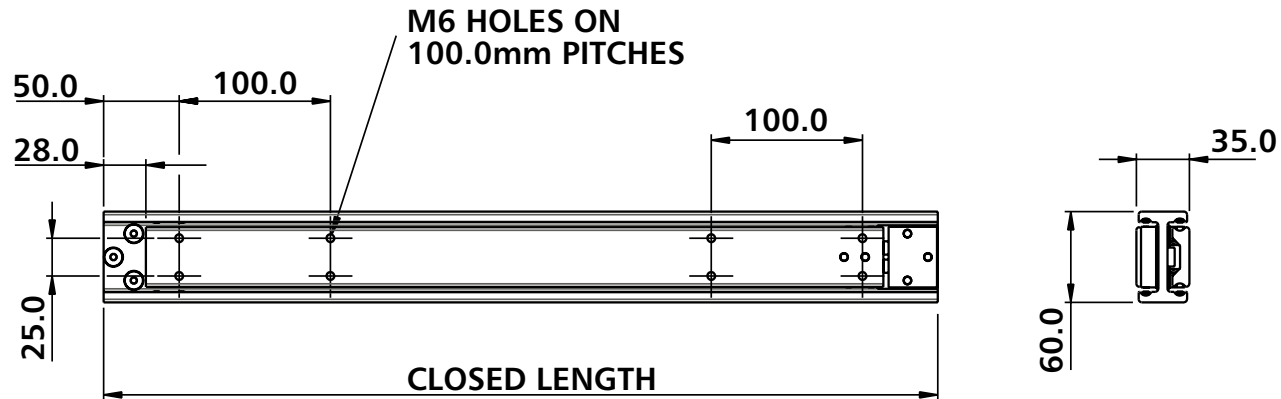
VIEW OF SLIDE WHEN CLOSED INNER/OUTER BEAMS ARE IDENTICAL
